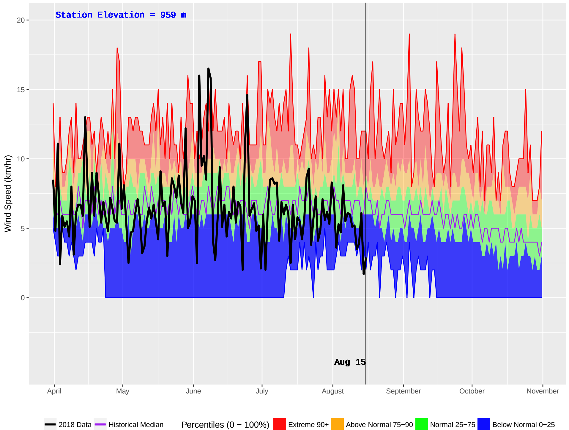
WELLS GRAY (266) : Historical (1994–2016) and Current (2018) Daily Wind Speed
