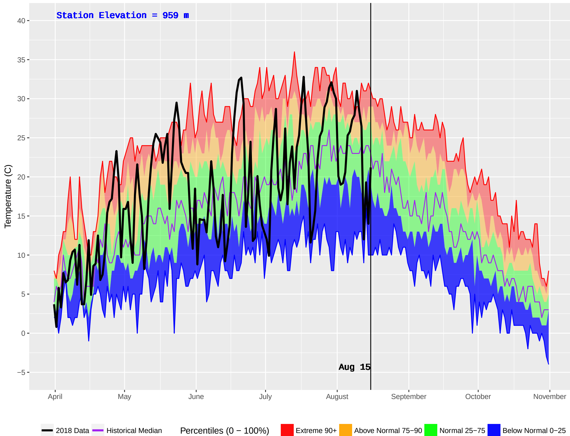
WELLS GRAY (266) : Historical (1994–2016) and Current (2018) Daily Temperature
