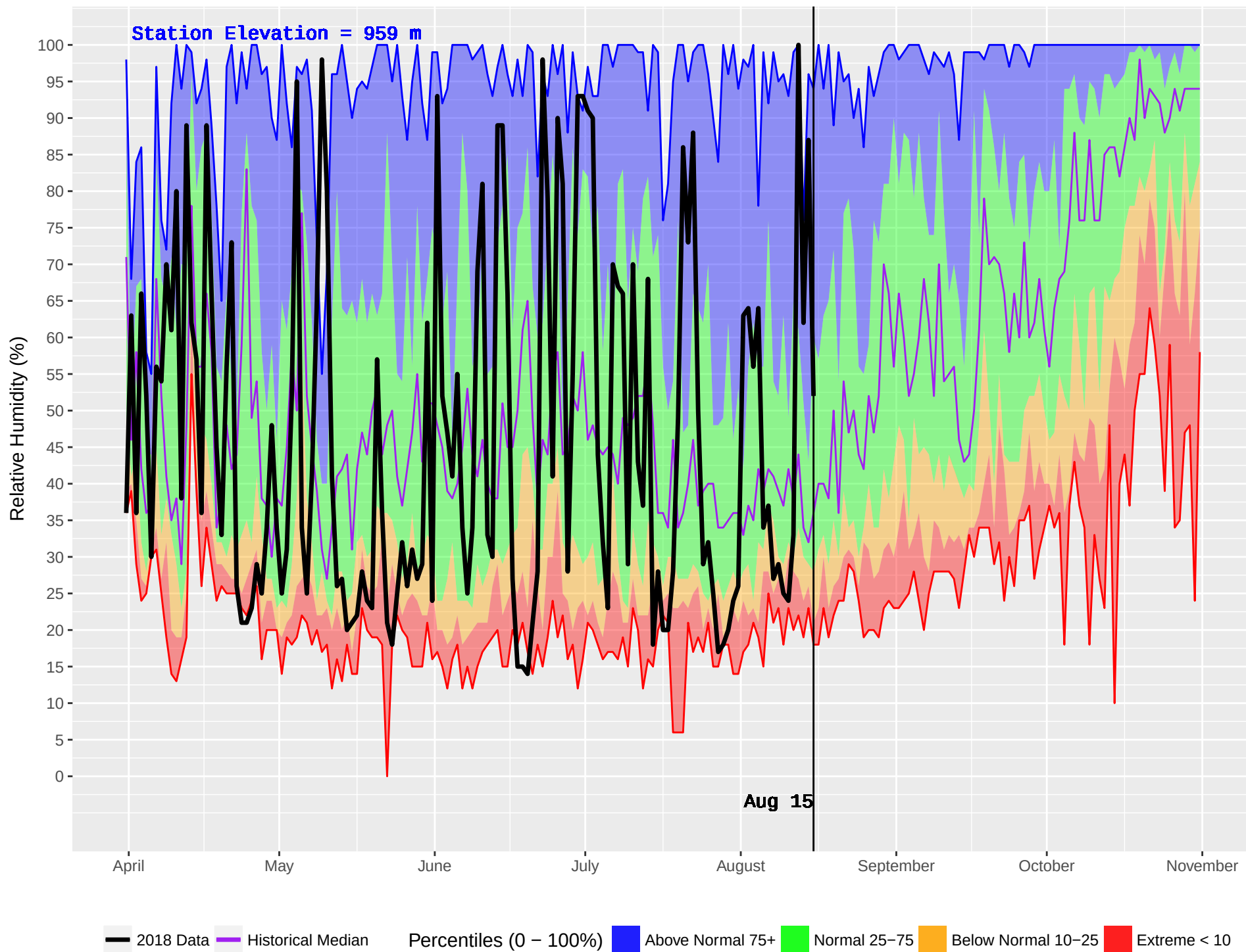
WELLS GRAY (266) : Historical (1994–2016) and Current (2018) Daily Relative Humidity
